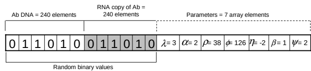
Fig. 3. Ab chromosome (DNA \cup RNA \cup parameters)
