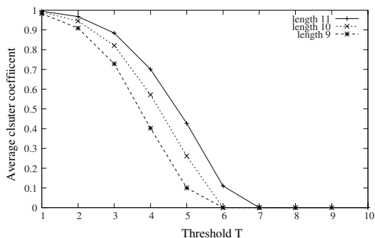
Fig. 1. The graph shows the average cluster coefficient in a potential network created by a bistring of length L with increasing threshold T
