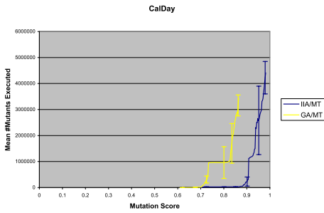
Fig. 3. Mean number of mutant executions to achieve at least a specific mutation score for the CalDay program
