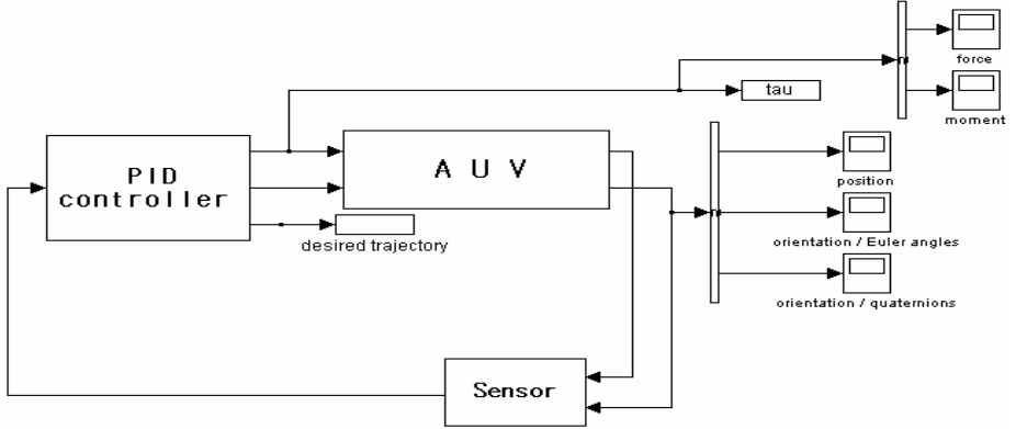
Fig. 2. Block diagram of the 6-DOF PID controller
