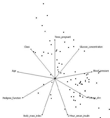
Fig. 6. Antibodies from Diabetes database after suppression and 60-40% split
