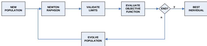
Fig. 1. Diagram Solution of a Population-Based Method
