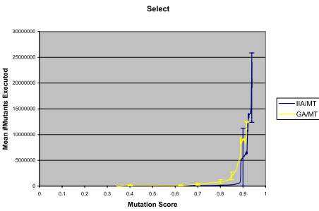
Fig. 5. Mean number of mutant executions to achieve at least a specific mutation score for the Select program
