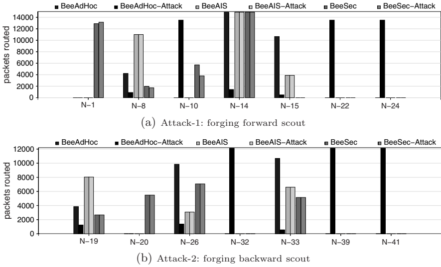
Fig. 4. Attacks: forging forward scout and forging backward scout
