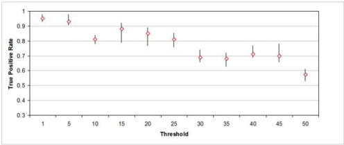
Fig. 10. True Positive Rate for testing data-set (type-2)
