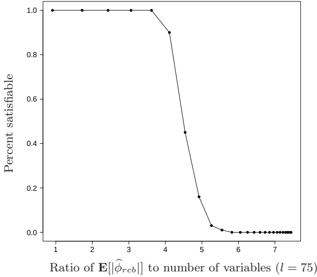
Fig. 3. Coherence between the percentage of satisfiable instances and the ratio of \mathbf{E}[|\hat{\phi}_{rcb}|]/l . The “hardest” instances live in the region where the number of satisfiable and unsatisfiable instances is equal, or in other words, the probability of instances being satisfiable equals 0.5.
