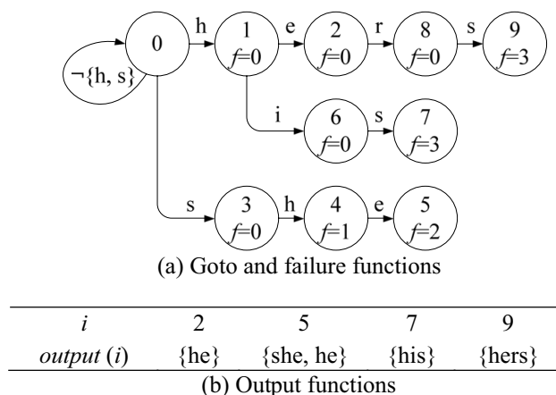
Fig. 1. The pattern matching machine constructed for the set of keywords {he, she, his, hers}. This example is extracted from [1]. The state nodes of this machine are numbered as from 0 to 9. The state 0 is designated as the start state. The goto and failure functions are illustrated in Fig. 1 (a), and the output functions are given in Fig. 1 (b).
