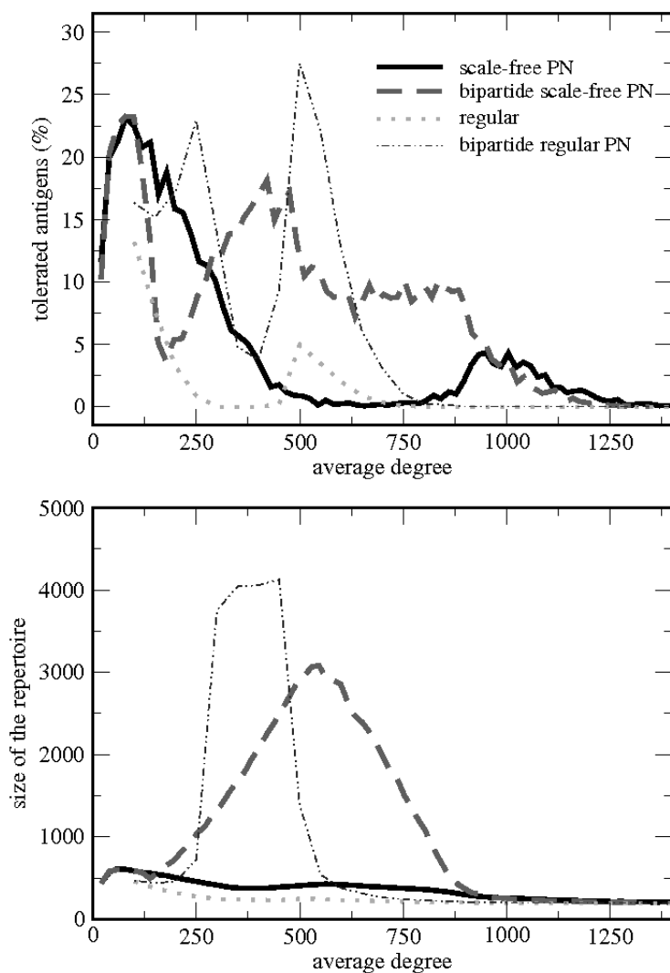
Fig. 4. The graphs show the results of simulation using a number of heterogeneous and homogeneous potential networks (both regular and bipartite in each case), as the potential average degree of the networks are varied
